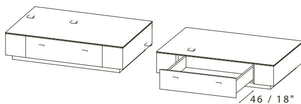
T163A 143X103XH.30 / 56X41XH.12" Drawer inner dimensions: 89X54XH.12 / 35X21XH.5"
