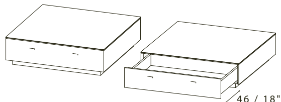
T161A 103X103XH.30 / 41X41XH.12" Drawer inner dimensions: 89X54XH.12 / 35X21XH.5"
