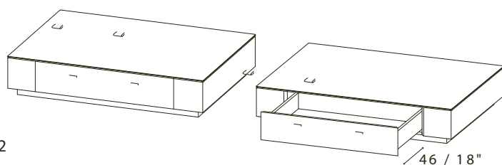
T163A 143X103XH.30 / 56X41XH.12" Drawer inner dimensions: 89X54XH.12 / 35X21XH.5"
